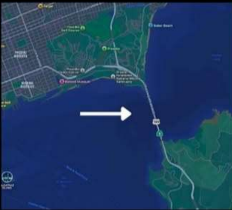
Input Image
